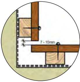
DETAIL 7.
