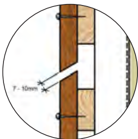
DETAIL 12.
